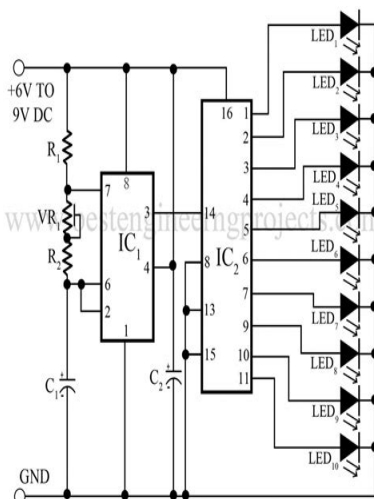
Figure 1: Circuit Diagram of LED Chaser
